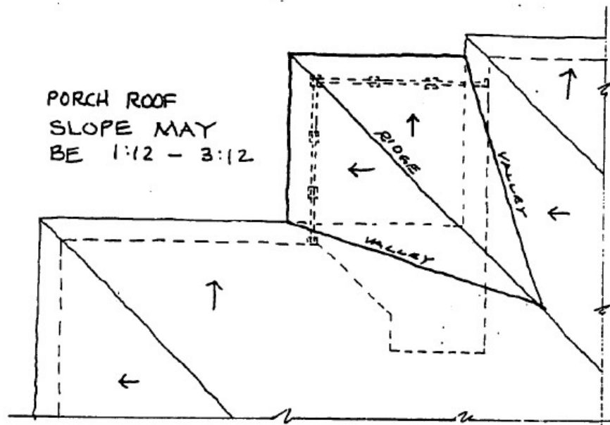
ROOF PLAN
